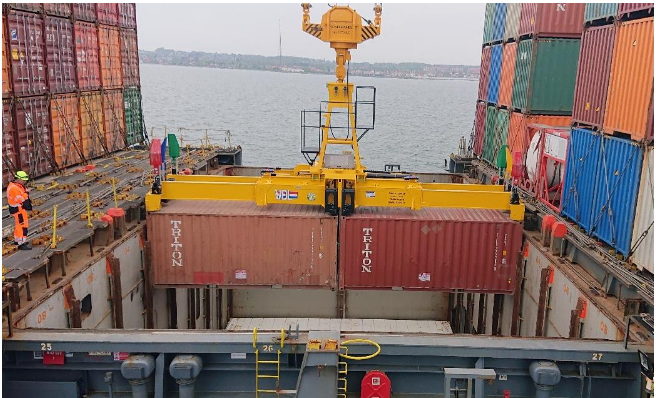
The new VDL CH6650FT spreader in service at the APM-terminal in Port of Kalundborg
